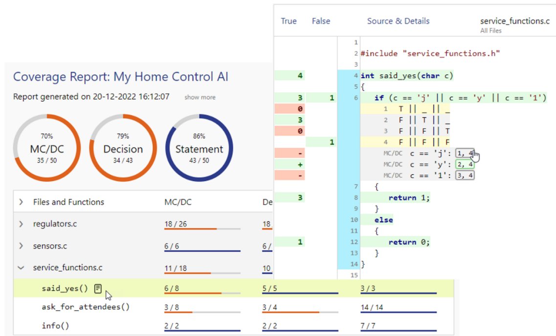
Fig. 1 : In addition to an overview of the code coverage of the individual code parts, Testwell CTC++ also displays detailed information that shows exactly to what extent the source code is covered by tests, even for the highest coverage levels.
